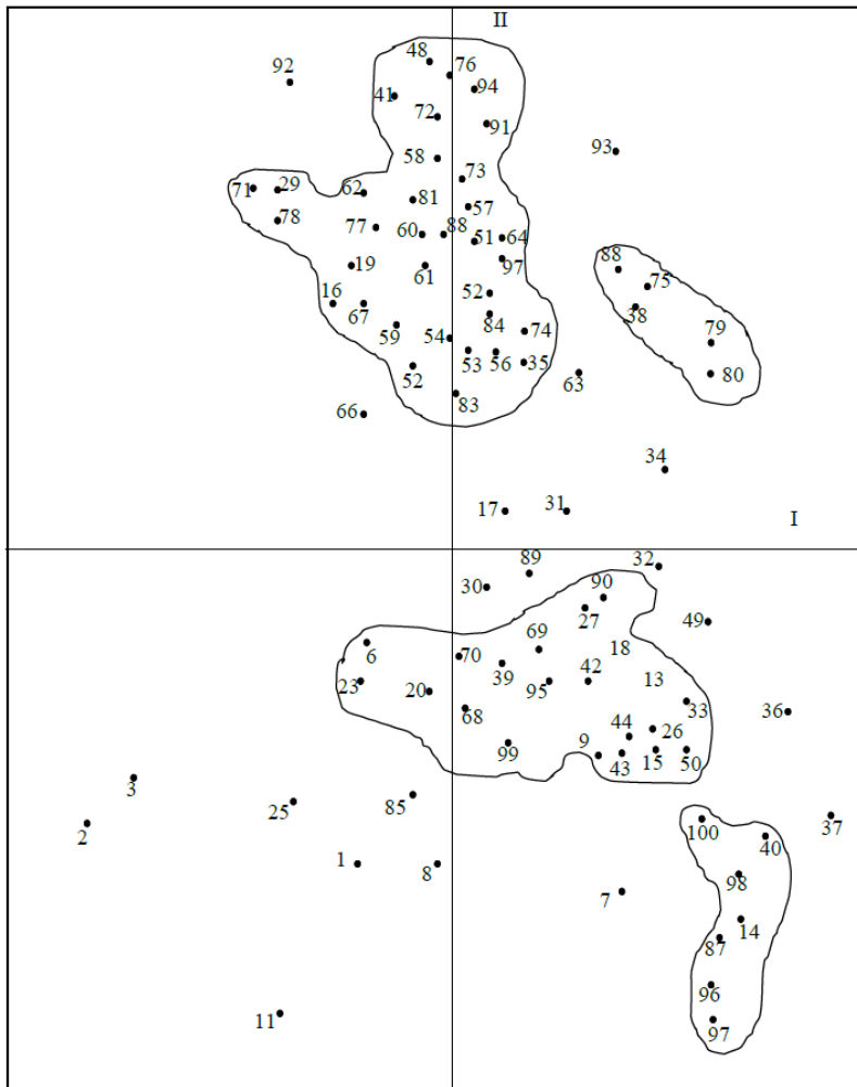
Fig. 3: Physiognomic Ordination
