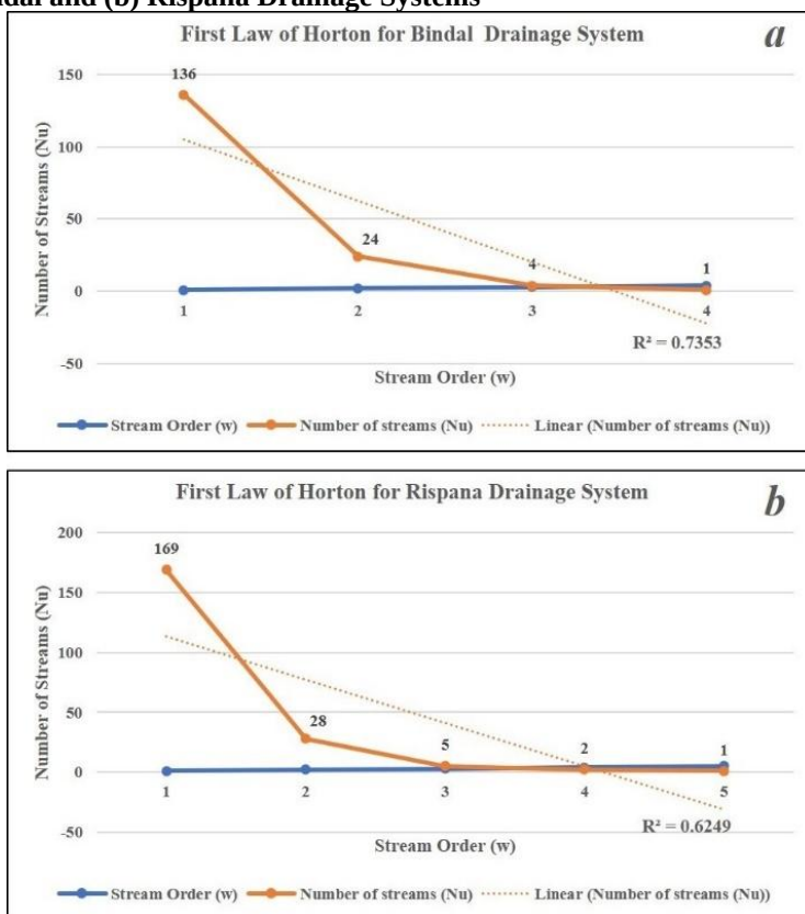
Fig. 3: Graphical Representation of Number of Streams (Nu) and Stream Order (w) for the (a) Bindal and (b) Rispana Drainage Systems
